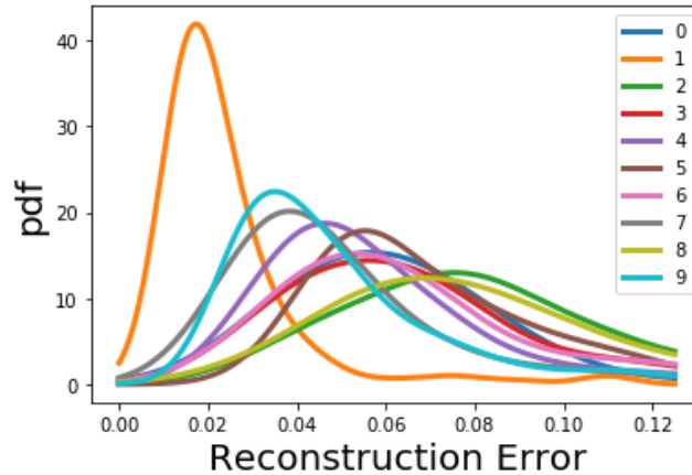
Fig. 2: Probability density function of reconstruction errors associated with different classes of training samples, estimated via kernel density estimation.
